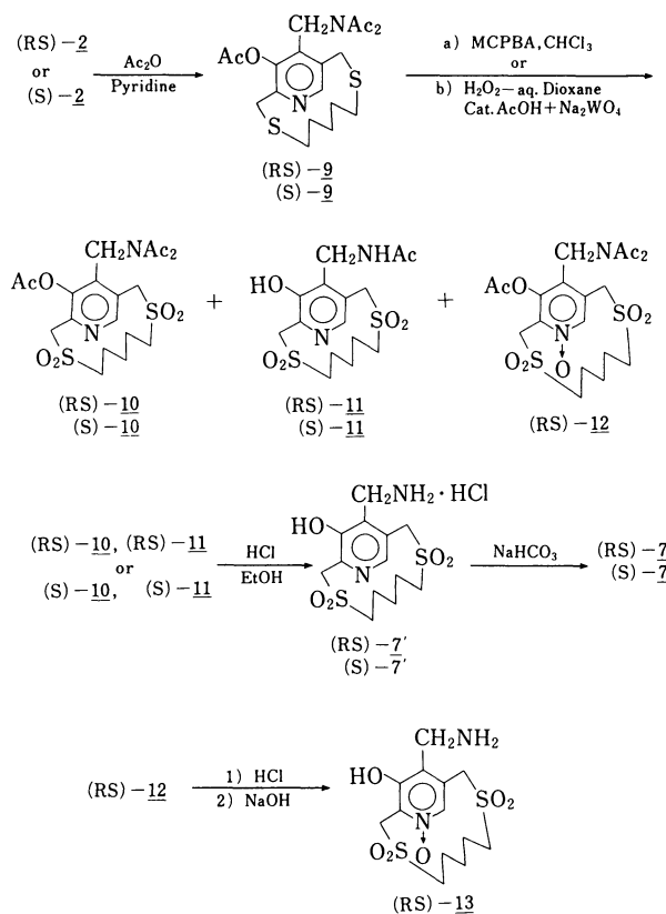
Scheme 5.
